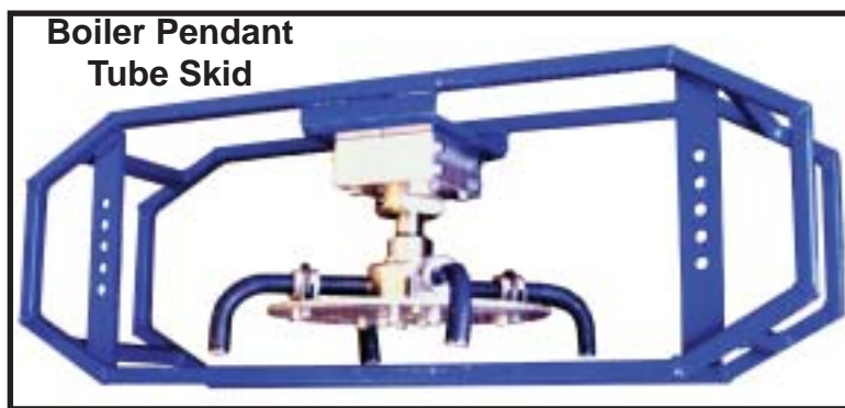
Examples of custom systems based on the SG-30 Free Spinner
