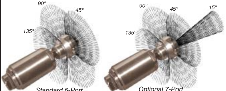
Standard 6-Port BJ 044-P4-6 Head APF4 Nozzle Tips
