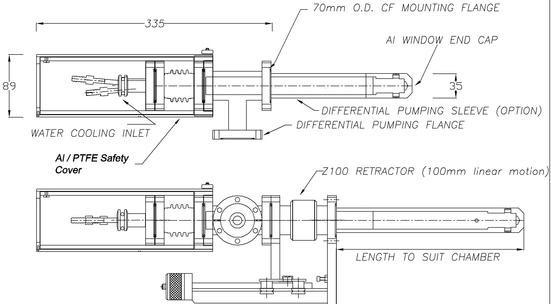
TX400 X-ray source shown with and without Z100 retractor Note: Insertion length is custom made to suit customers chamber
