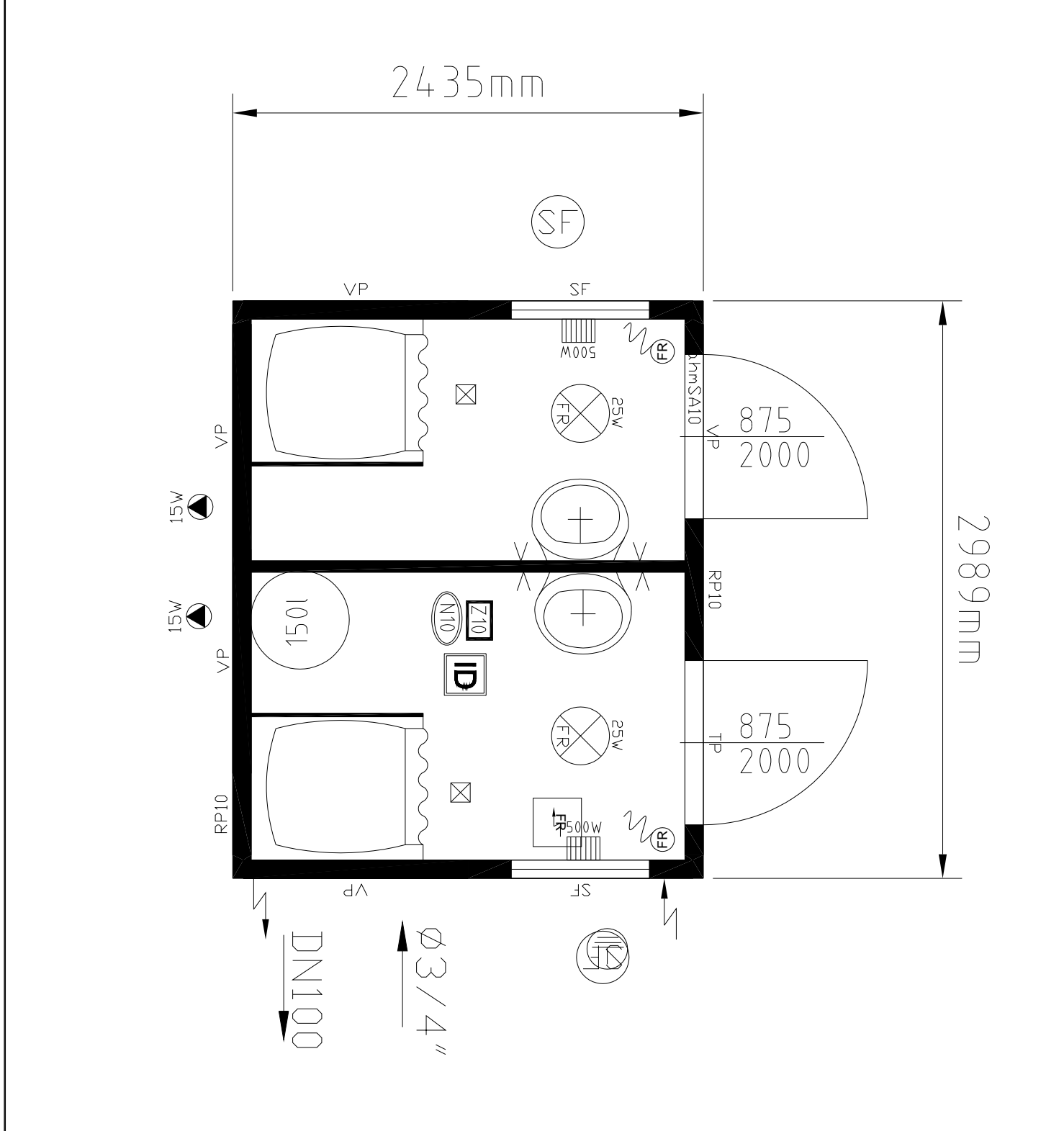
102542.dwg
